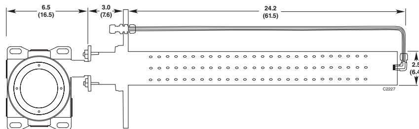
Figure 2—Dimensions of PIRDUCT Detector in Inches (cm)
